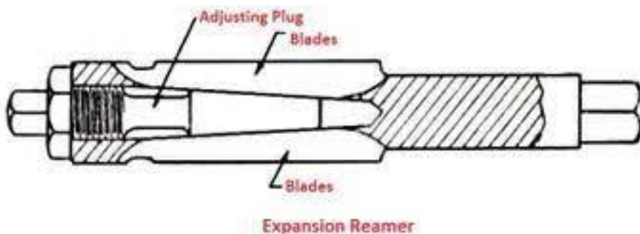
Expansion Reamer
